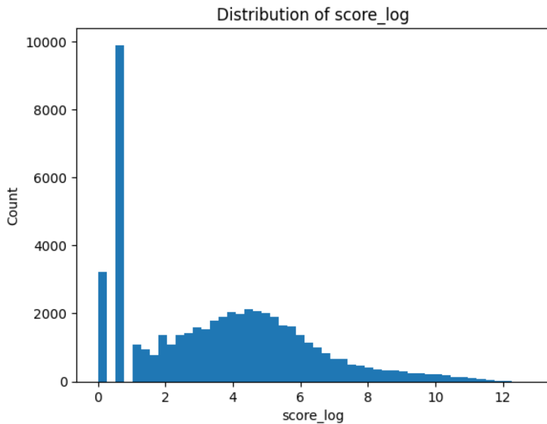
Figure 5. Log-transformed score distribution ( \text{score\_log} = \log_{10}(\text{score}) ) approximating a bell shape after transformation.
