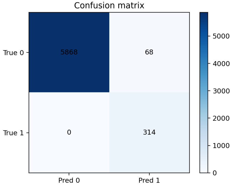
Figure 12. Confusion matrix for the full model at 0.5 threshold, showing the precision-recall tradeoff inherent in rare-event classification.
