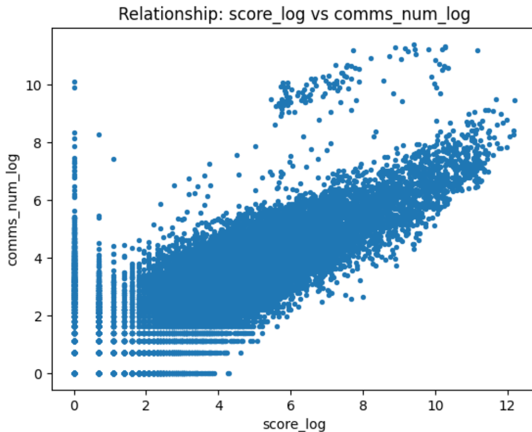
Figure 6. Scatter plot of score_log vs. comms_num_log showing strong positive association (Spearman rho = 0.79).
