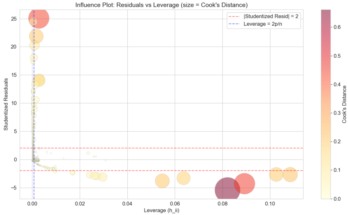
Figure A.2. Cook's Distance vs. leverage influence plot for engagement regression diagnostics.
