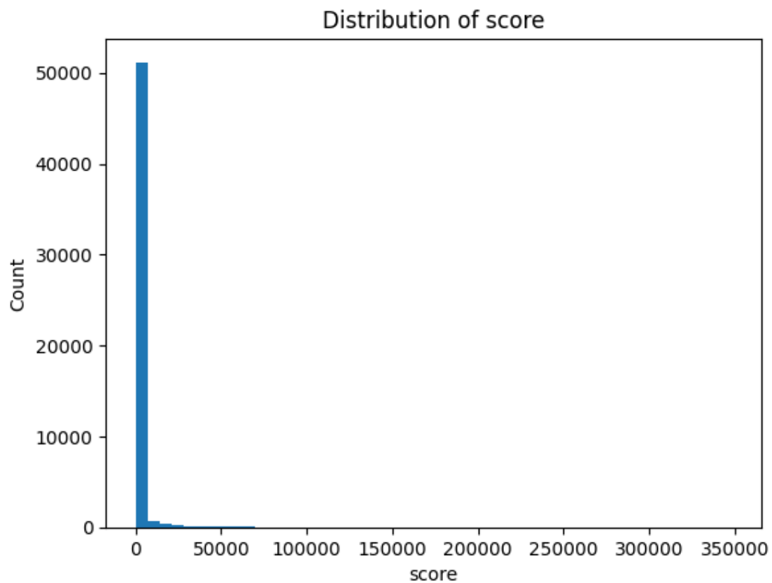
Figure 4. Raw score distribution showing extreme right skew with viral outliers orders of magnitude above the median.
