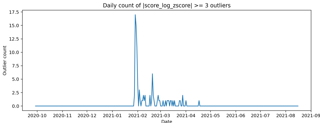
Figure 8. Daily count of statistical outliers ( |z| \geq 3 ) showing concentration during the January 2021 meme-stock event.
