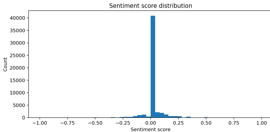
Figure 9. Distribution of domain-specific sentiment scores across all posts; the narrow range around zero reflects WSB’s ironic language limiting lexicon-based polarity detection.
