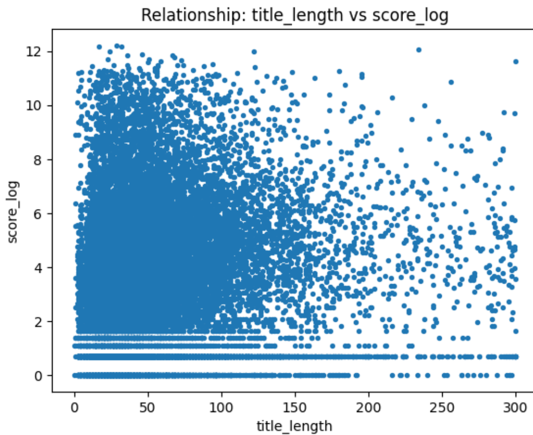
Figure A.12. Scatter plot of title length vs. score_log showing weak association, motivating richer text features.
