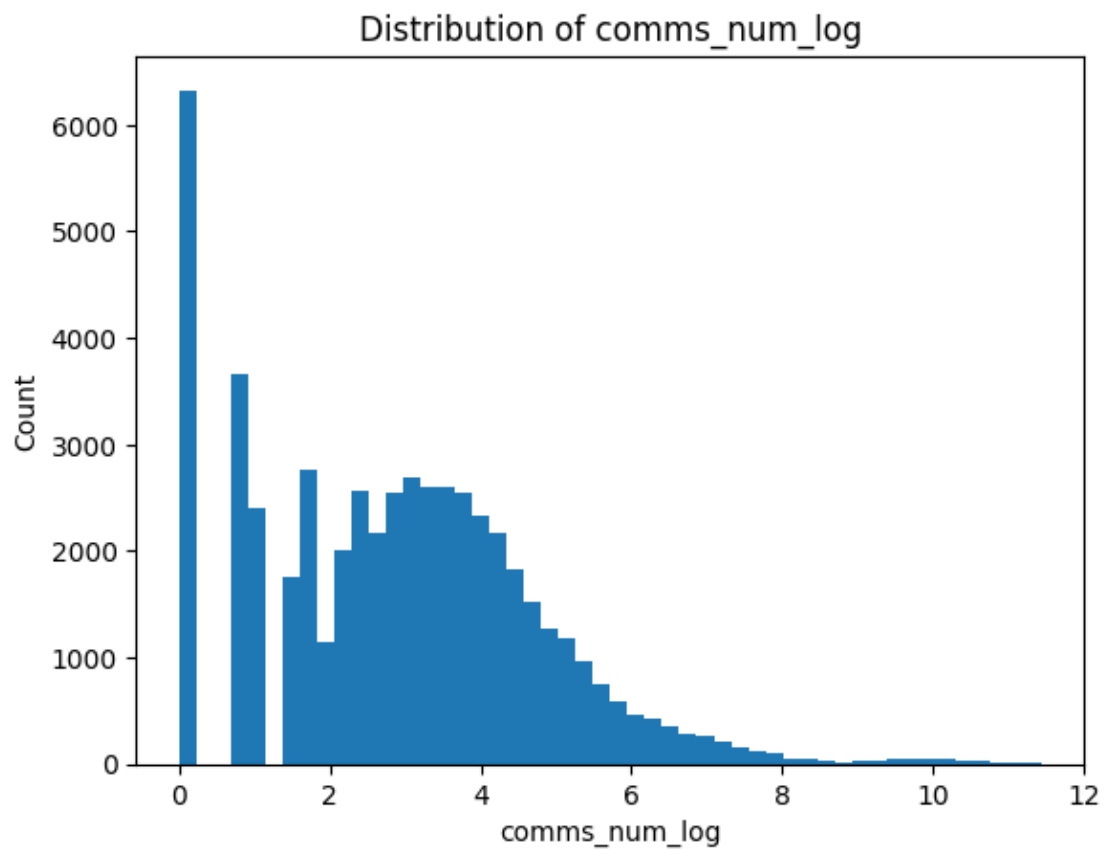
Figure A.6. Log-transformed comment count distribution showing approximate normality after \log_{1p} .
