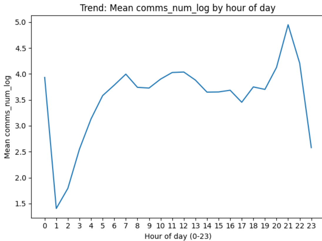
Figure A.14. Mean comms_num_log by posting hour; comment engagement follows a similar hourly pattern to score.
