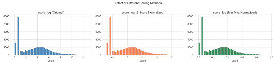
Figure 3. Comparison of z-score and min-max scaling for numerical features, ensuring comparable model inputs.
